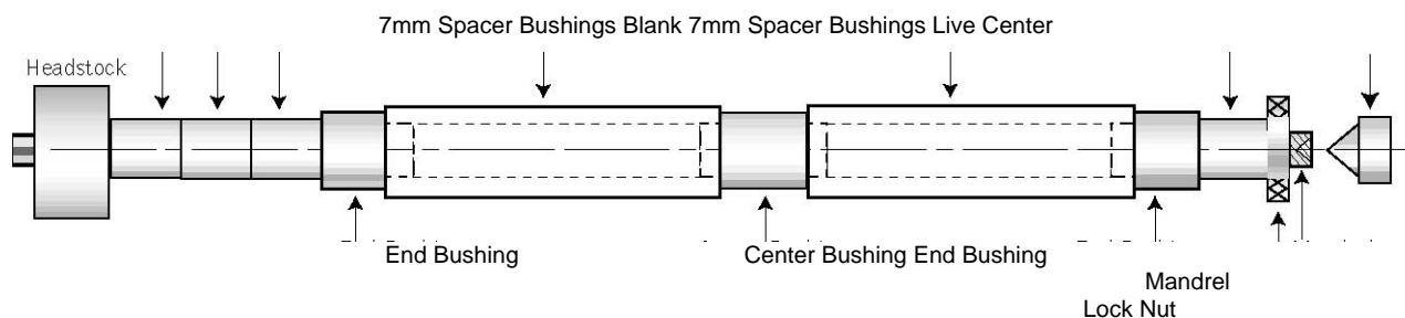
Diagram C: TURNING THE BLANKS
