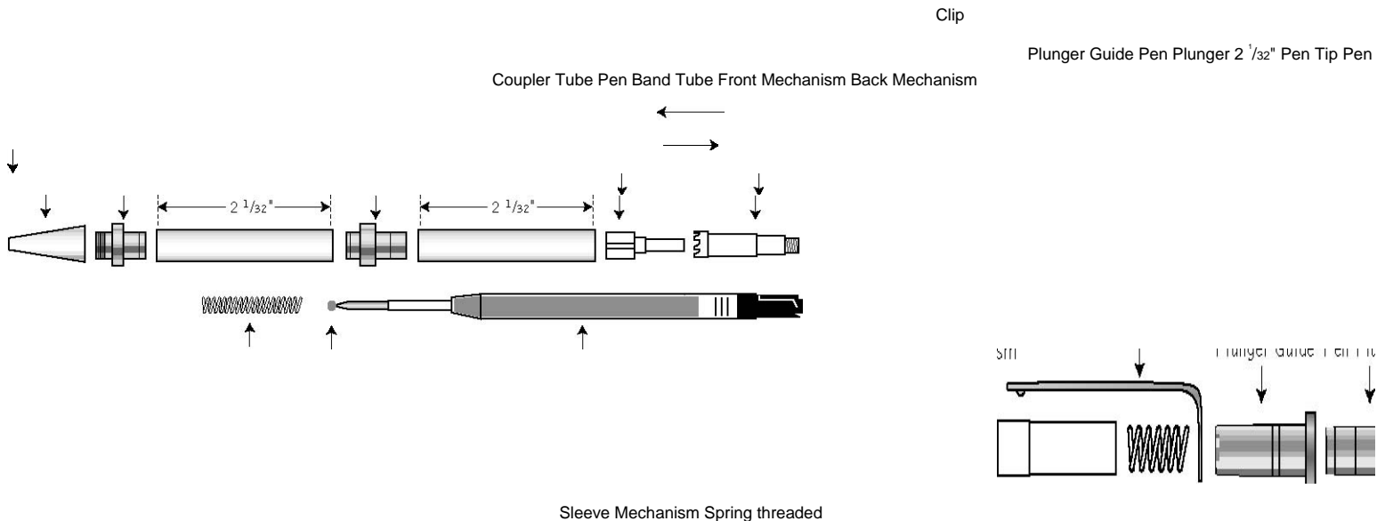
Diagram A: PEN PARTS
