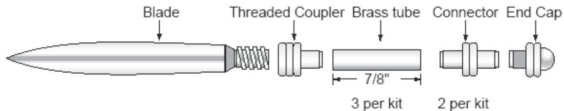
Diagram B - Letter Opener Parts
